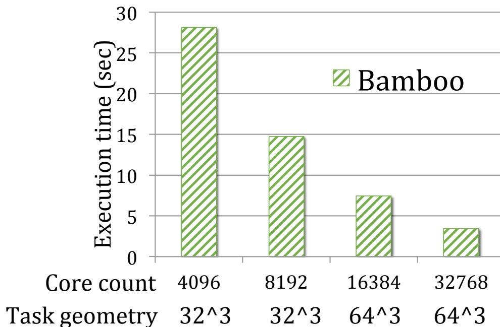
Figure 7.6. A strong scaling study on Hopper. We fixed the problem size at 1472^3 . Bamboo allows LULESH to be run on an arbitrary number of processes.
